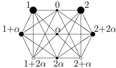
FIGURE 4. The unit graph G(\mathbb{Z}_3[x]/\langle x^2 \rangle) and its 4-colouring.
