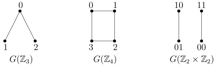
FIGURE 1. The unit graphs of some specific rings.
