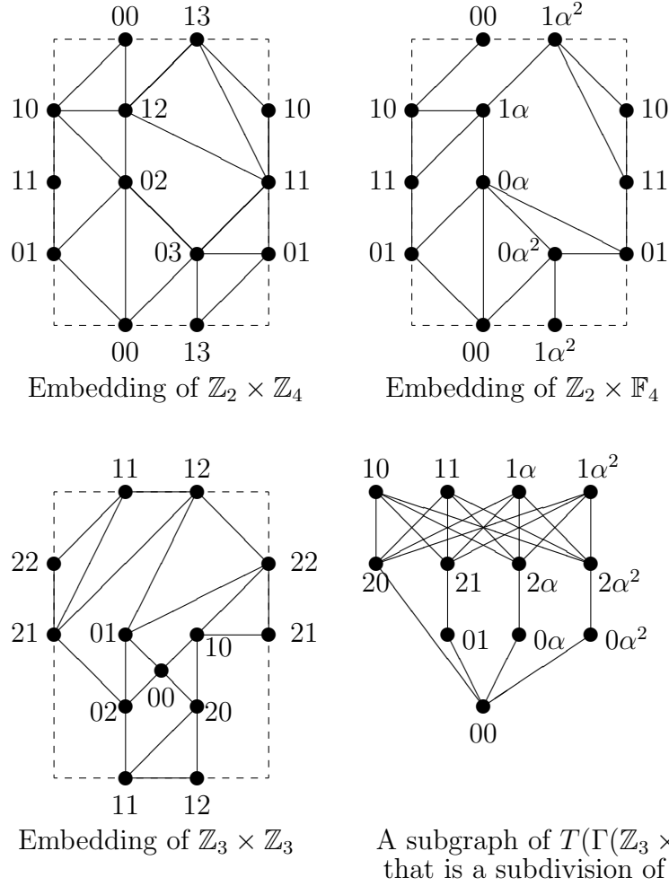
FIGURE 7. Embeddings in the torus and a subgraph of T(\Gamma(\mathbb{Z}_3 \times \mathbb{F}_4))
