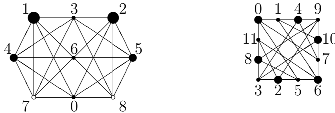
FIGURE 5. The unit graphs G(\mathbb{Z}_9) and G(\mathbb{Z}_{12}) and their four-coloring and two-coloring
