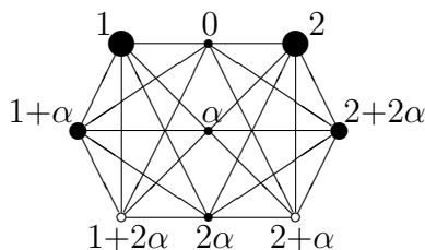
FIGURE 6. The unit graph G(\mathbb{Z}_3[x]/(x^2)) and its four-coloring
