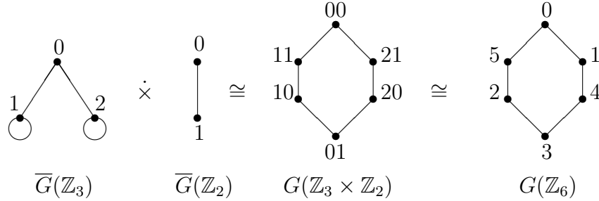
FIGURE 3. The category product of two closed unit graphs
